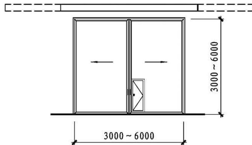
帶小門双向推拉门
